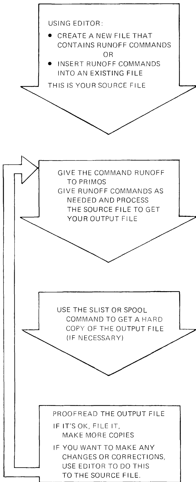
Figure 5-1 Using RUNOFF
